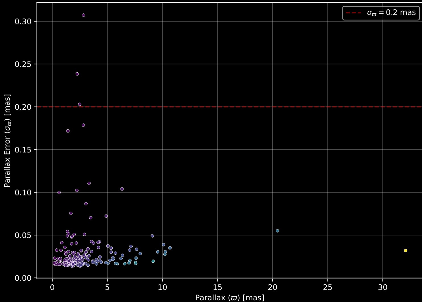
APOGEE DR17 Field: [126-55-O] Parallax Quality (n= 216)
