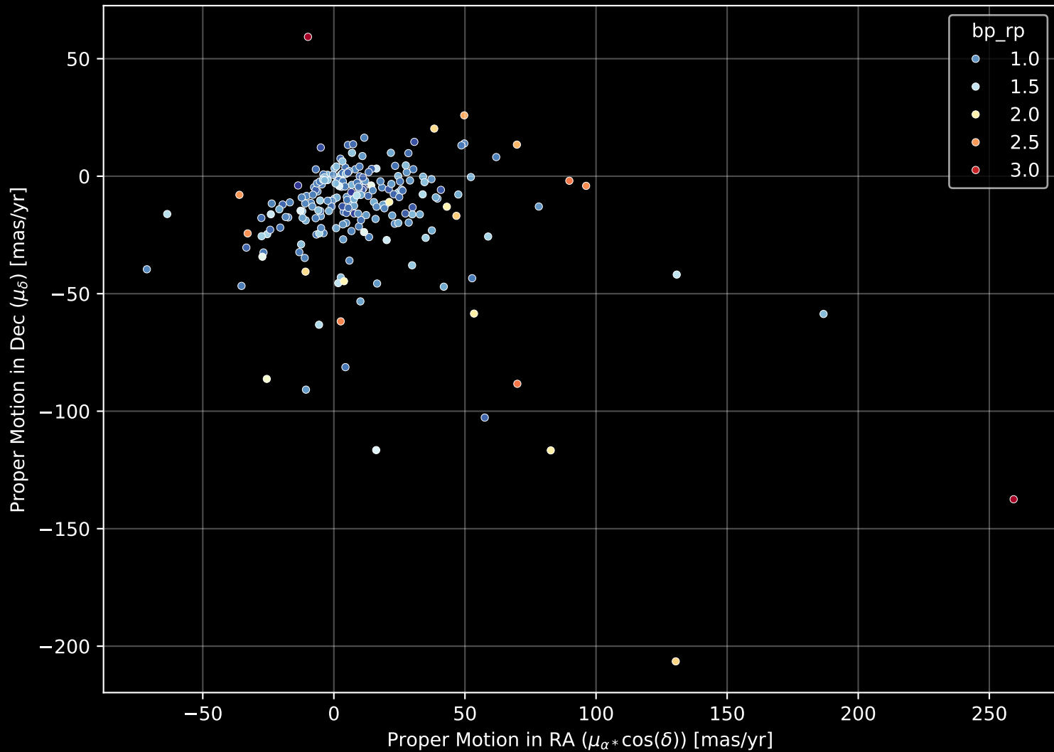
APOGEE DR17 Field: [126-55-O] Proper Motion Diagram (n= 216)
