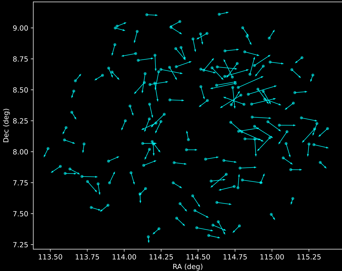
APOGEE DR17 Noise Stream Proper Motion Vectors (n=143)
