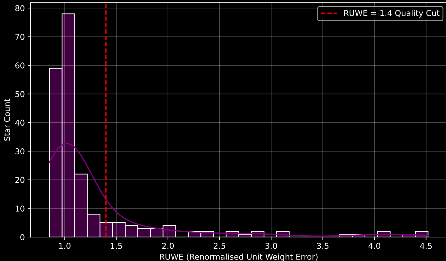
GAPOGEE DR17 Field [126-55-O] RUWE Distribution (n= 209)
