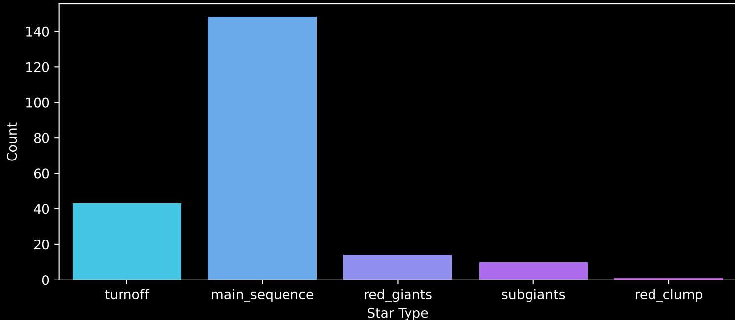
APOGEE DR17 Field: [126-55-O] Count plot of Star Type
