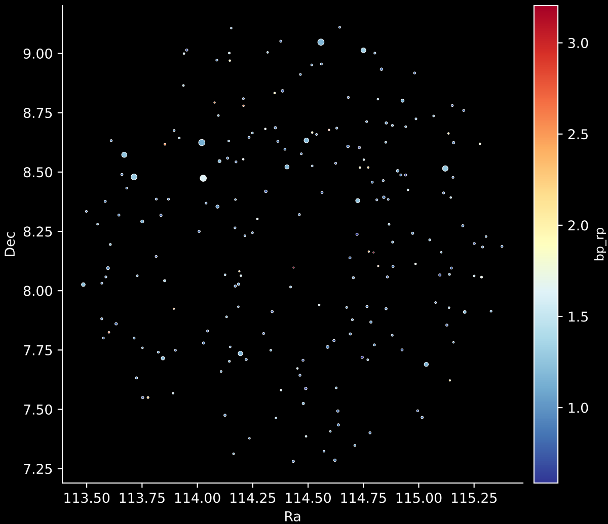
APOGEE DR17 Field: [126-55-O] Stars: 216
