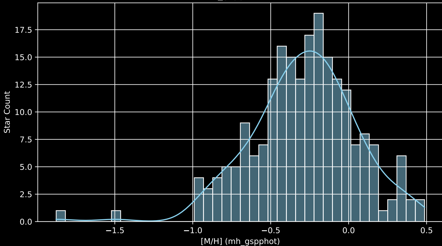
APOGEE DR17 Field: [126-55-O [M/H] (mh_gspphot) (n= 213)
